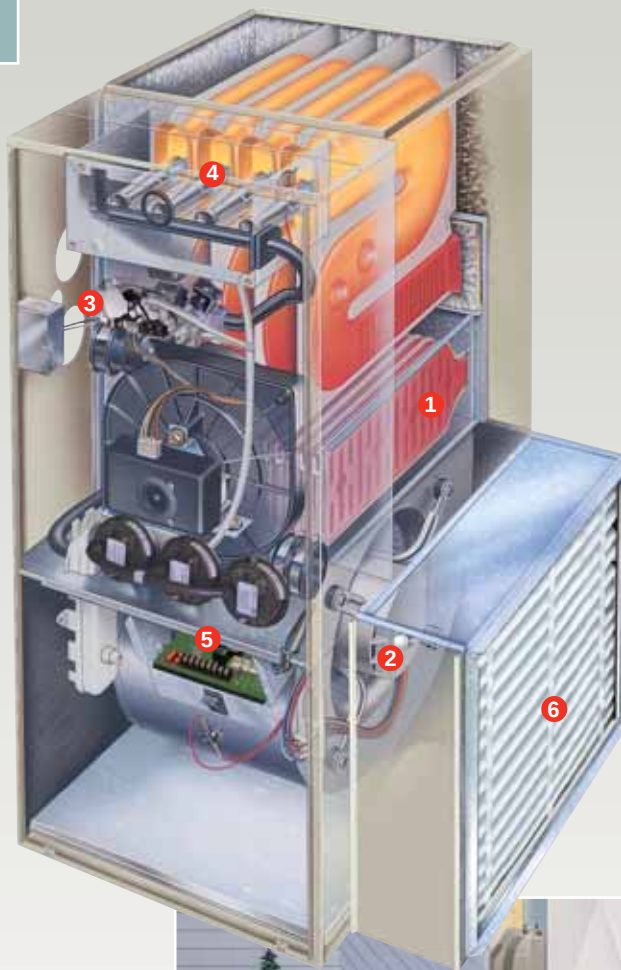
Model 355CAV shown with optional Bryant High-Efficiency Media Filter
